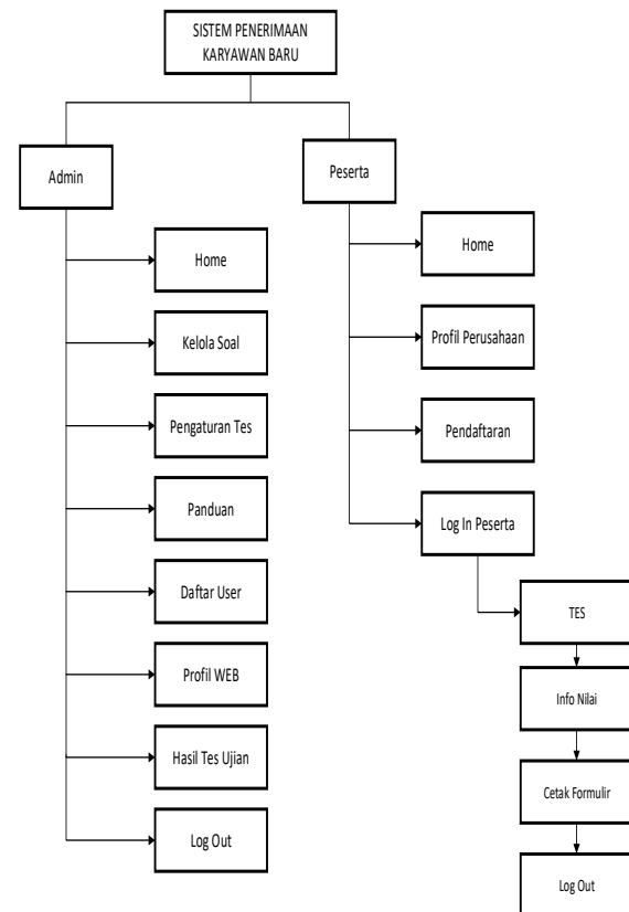
Gambar 4-4 HIPO (Hierarchy Input Process Output)
