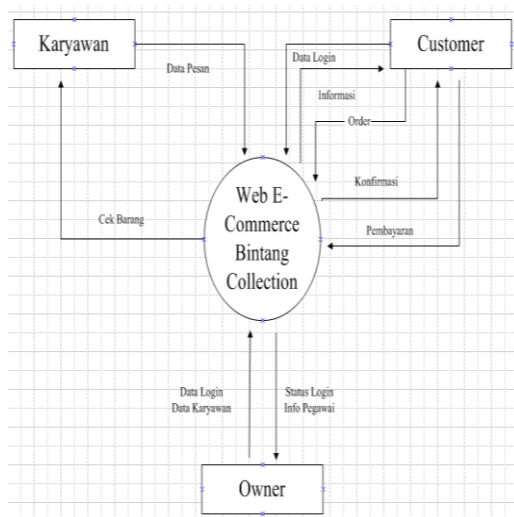
Gambar 3.6.2. Data Flow Diagram ( DFD )
